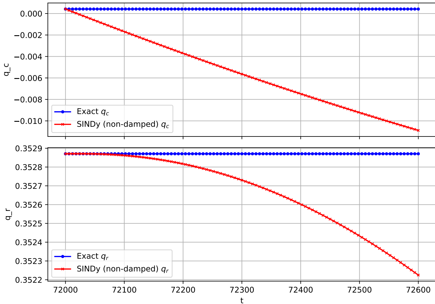
Trajectory 330 (non-damped)
