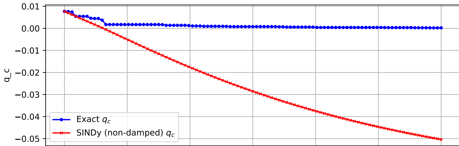
Trajectory 343 (non-damped)
