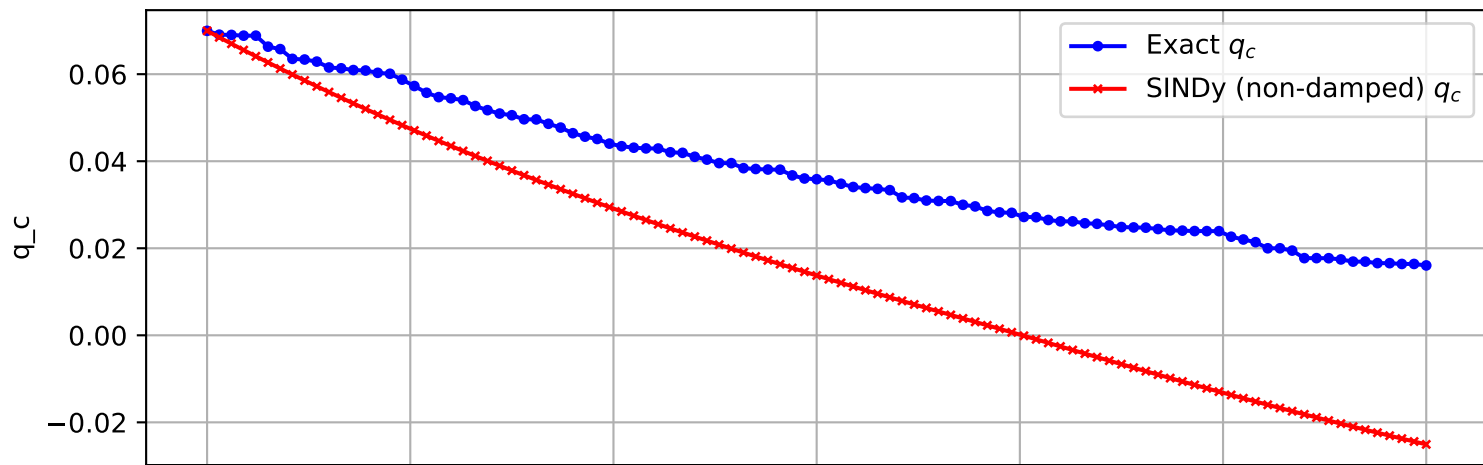
Trajectory 345 (non-damped)
