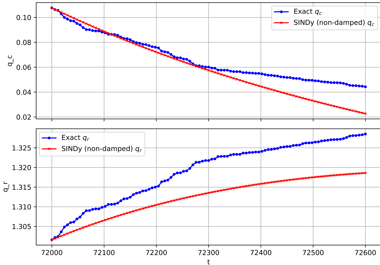
Trajectory 347 (non-damped)
