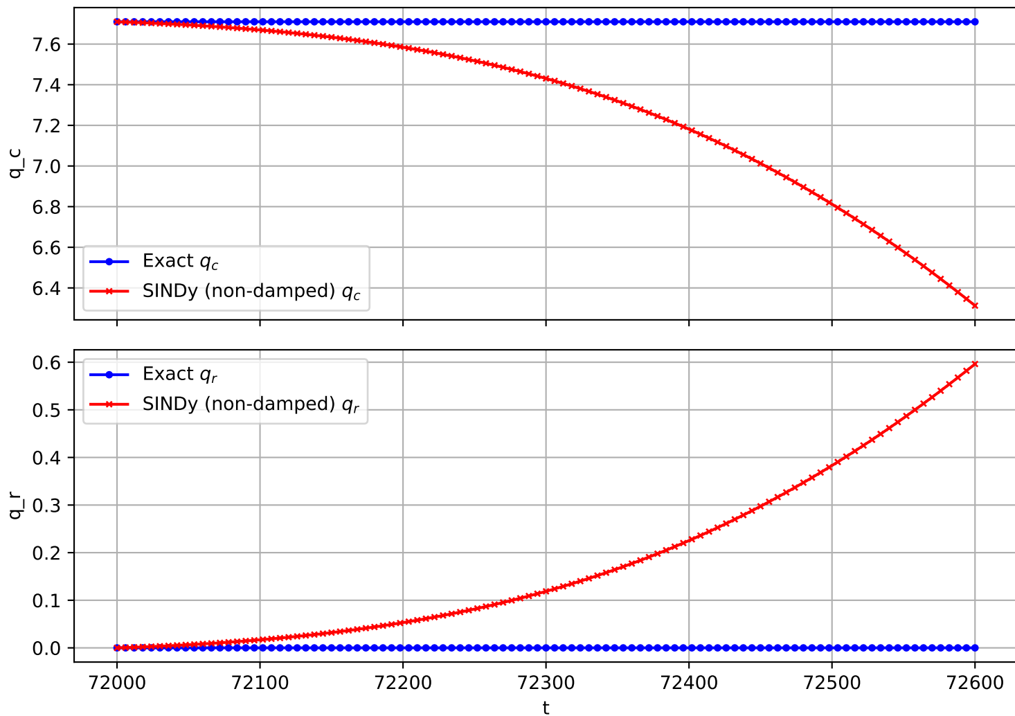
Trajectory 35 (non-damped)
