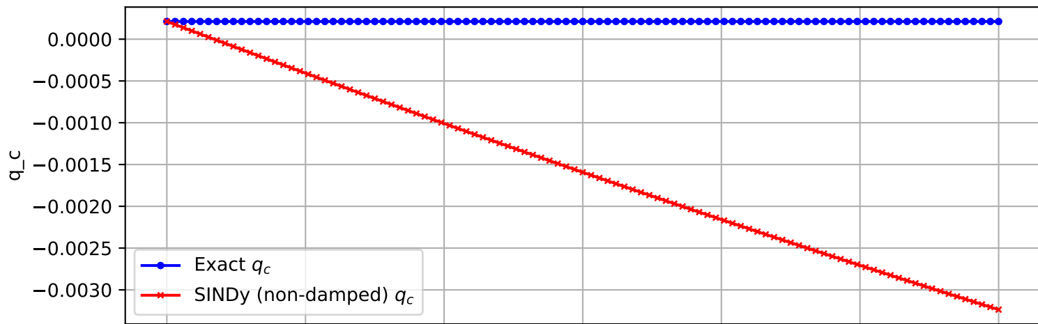
Trajectory 355 (non-damped)
