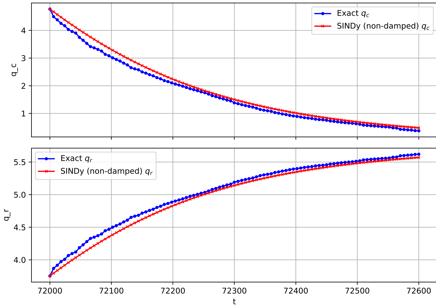
Trajectory 367 (non-damped)
