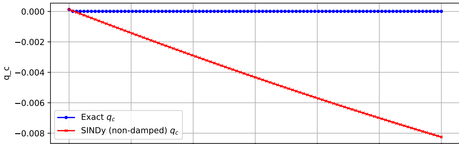
Trajectory 373 (non-damped)
