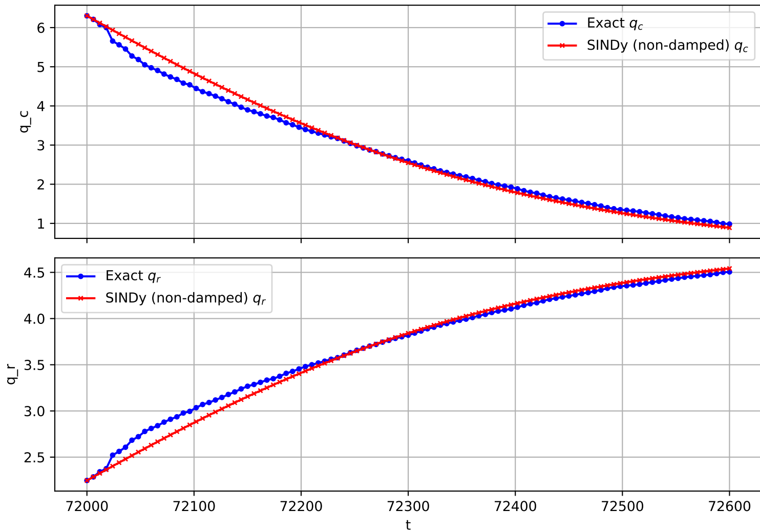
Trajectory 381 (non-damped)
