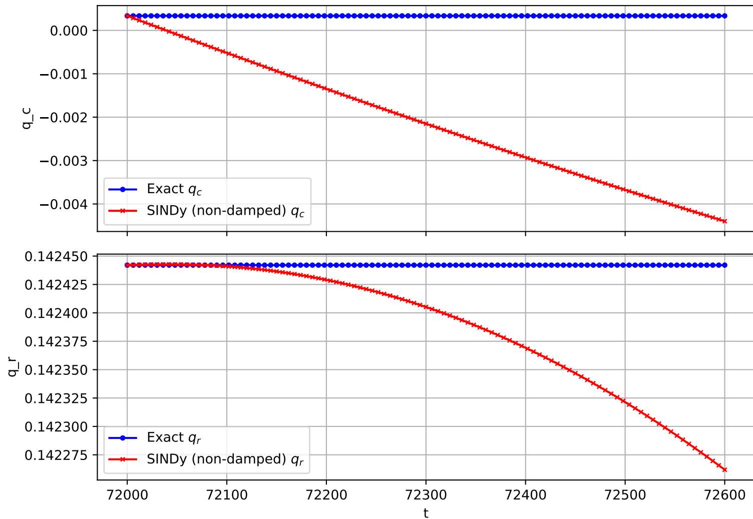
Trajectory 387 (non-damped)
