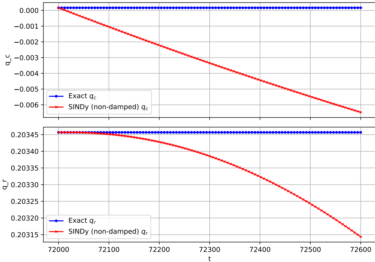
Trajectory 396 (non-damped)
