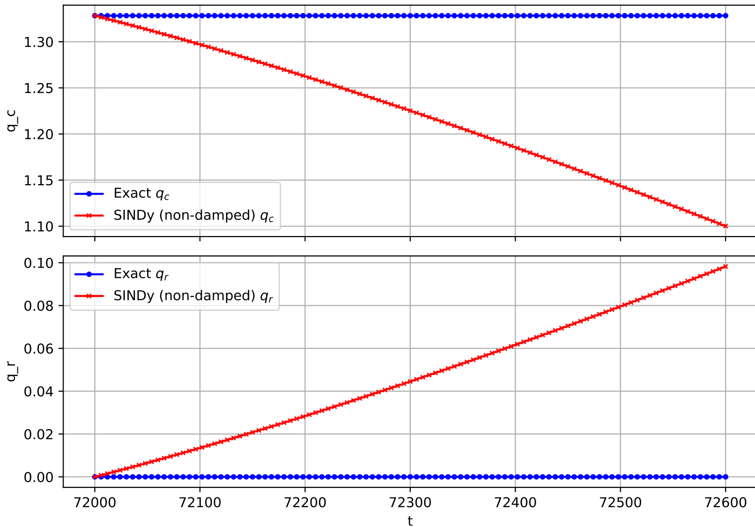
Trajectory 408 (non-damped)
