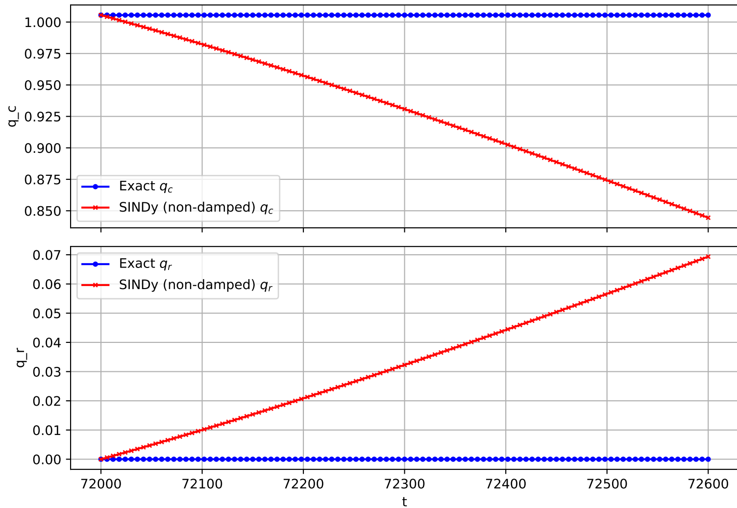
Trajectory 413 (non-damped)
