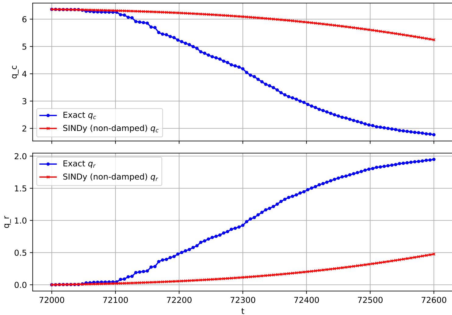
Trajectory 418 (non-damped)
