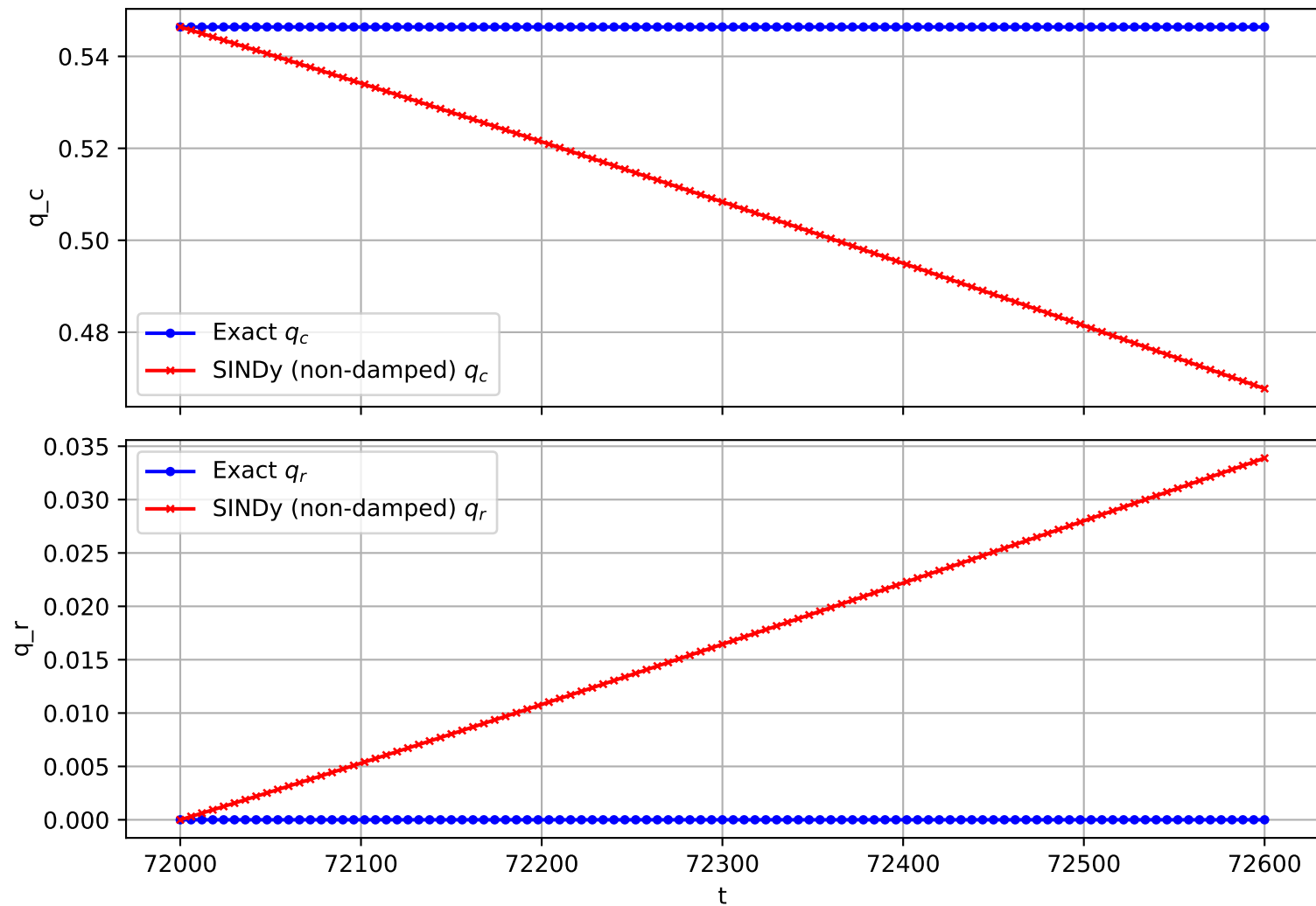
Trajectory 43 (non-damped)
