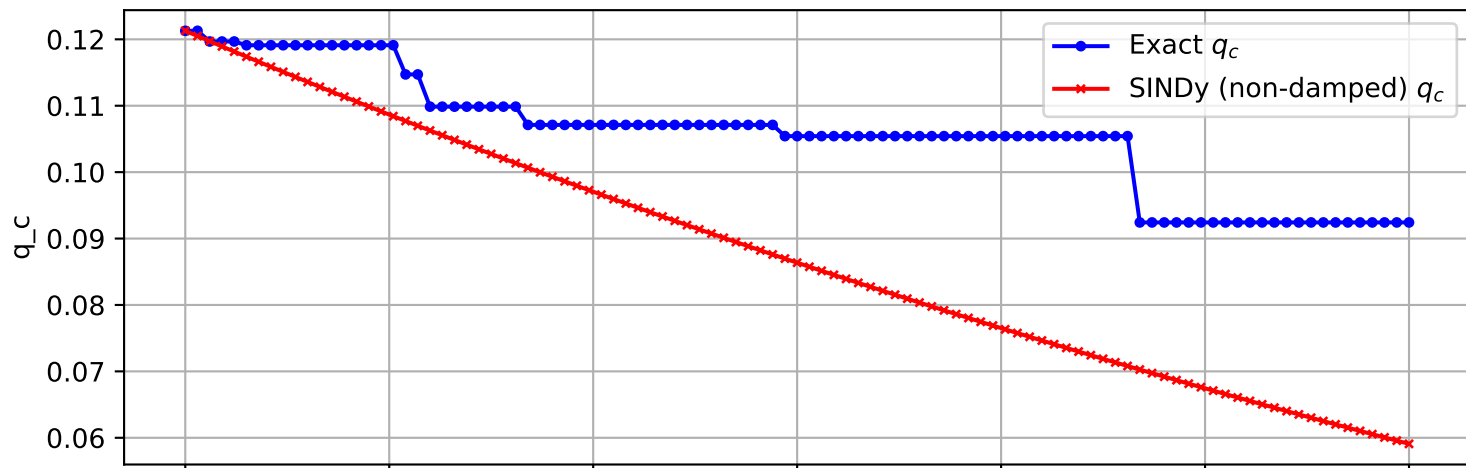
Trajectory 431 (non-damped)
