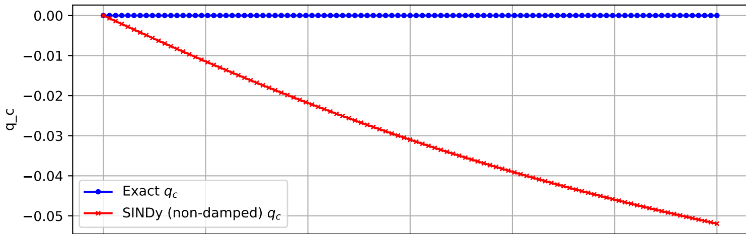
Trajectory 444 (non-damped)
