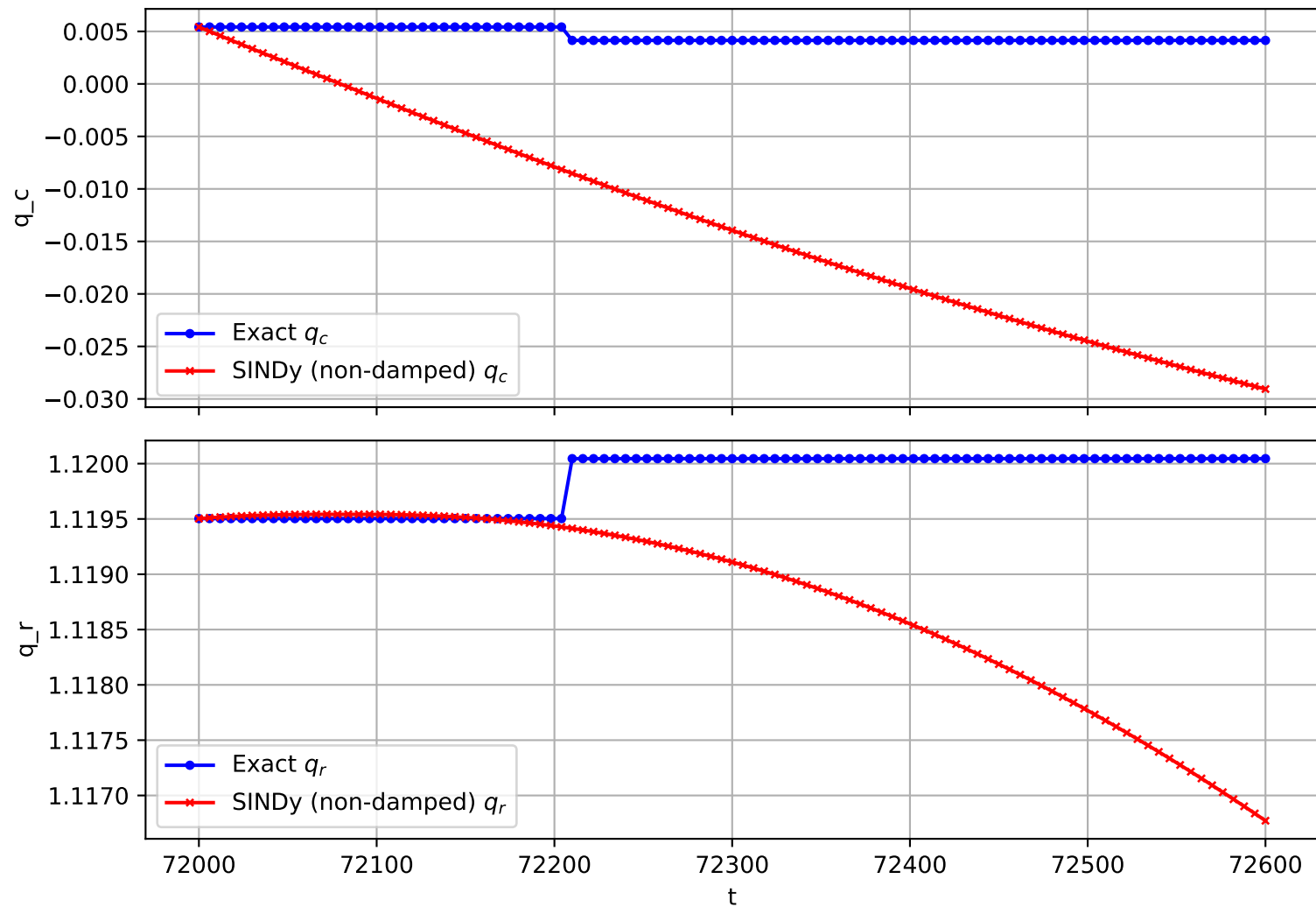
Trajectory 447 (non-damped)
