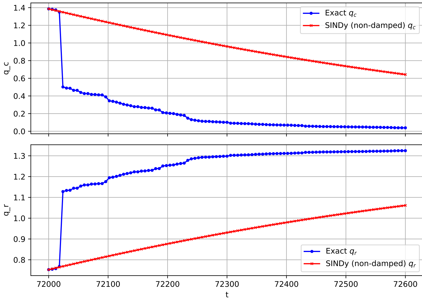
Trajectory 451 (non-damped)
