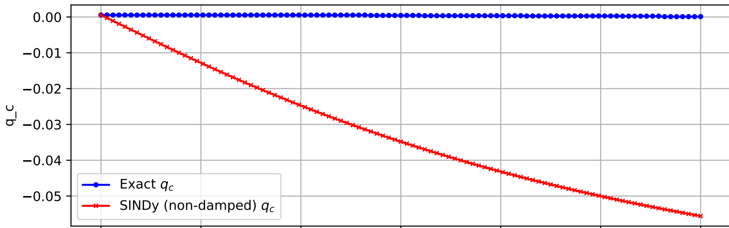
Trajectory 460 (non-damped)
