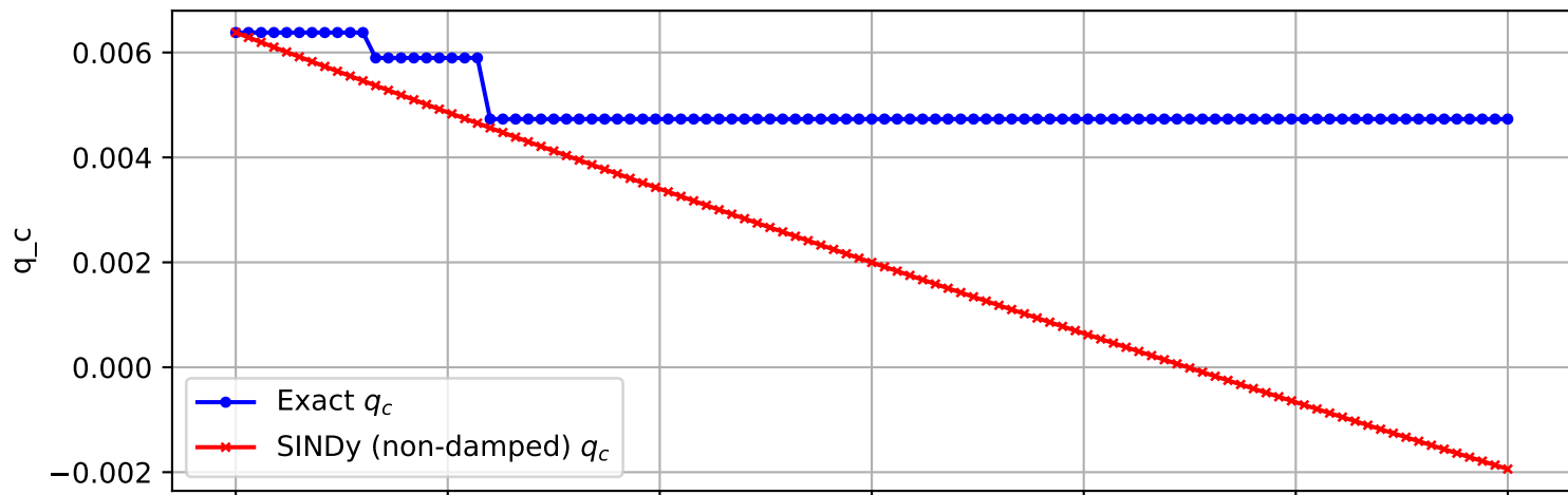
Trajectory 468 (non-damped)
