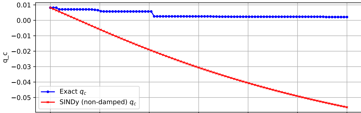
Trajectory 484 (non-damped)
