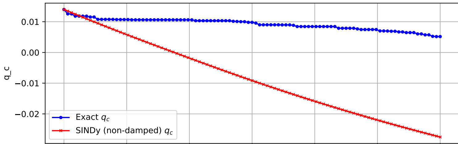
Trajectory 485 (non-damped)
