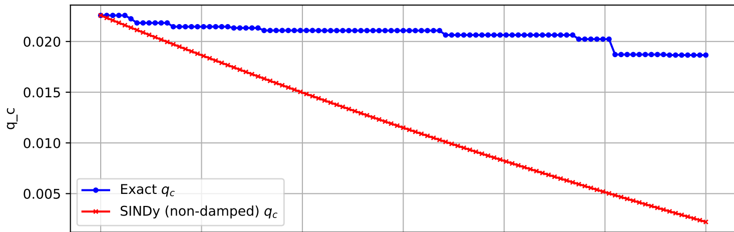
Trajectory 486 (non-damped)
