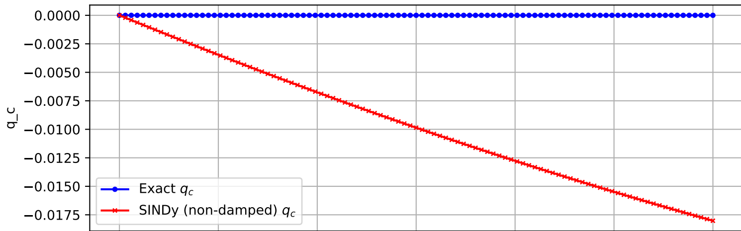
Trajectory 487 (non-damped)
