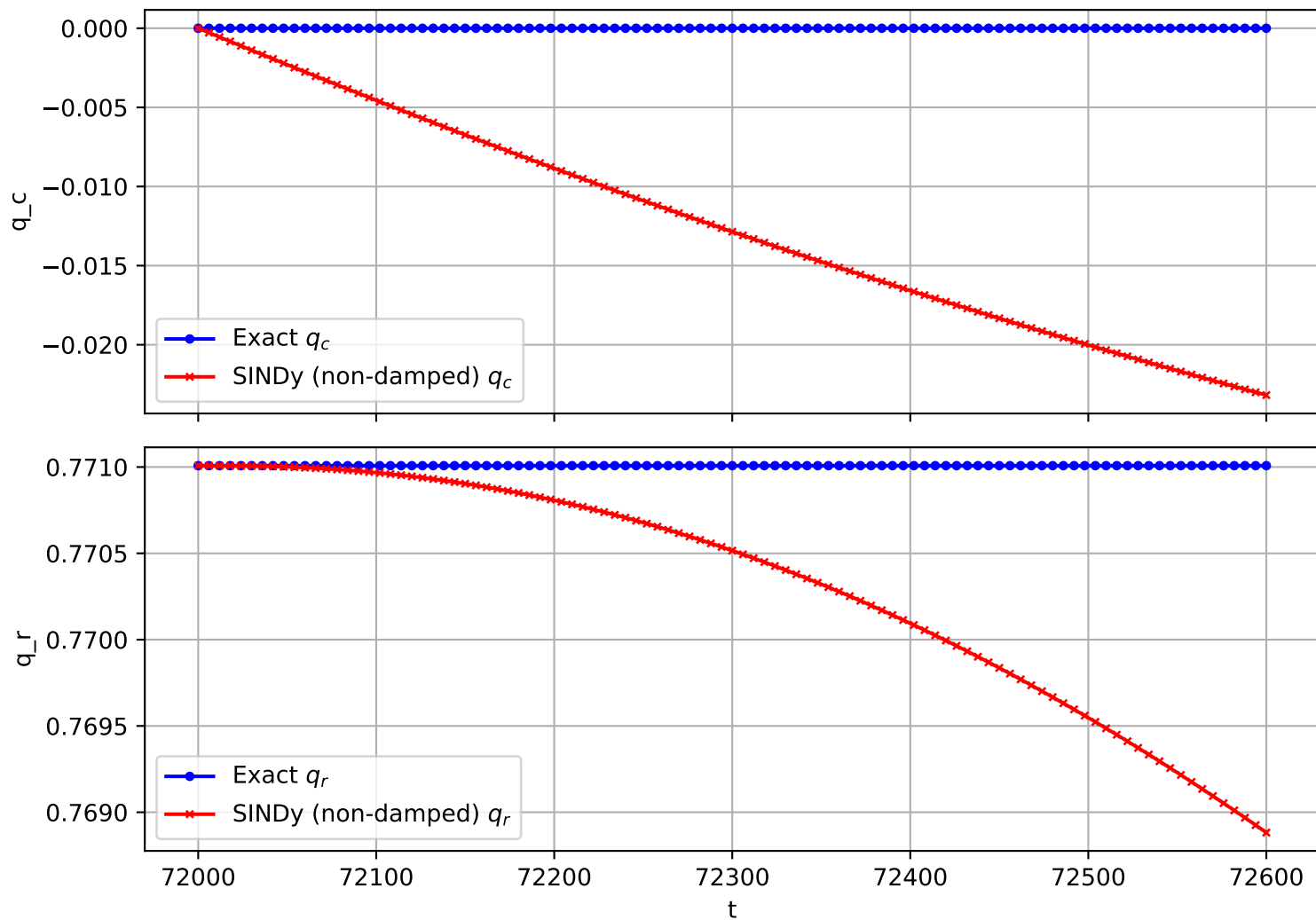
Trajectory 489 (non-damped)
