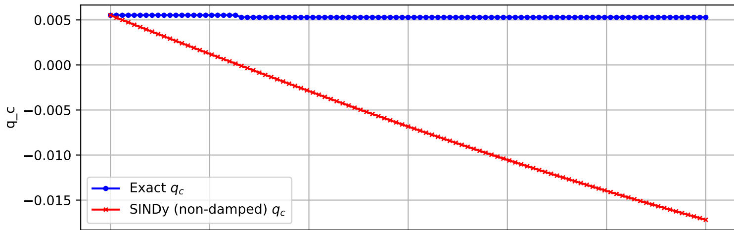
Trajectory 490 (non-damped)
