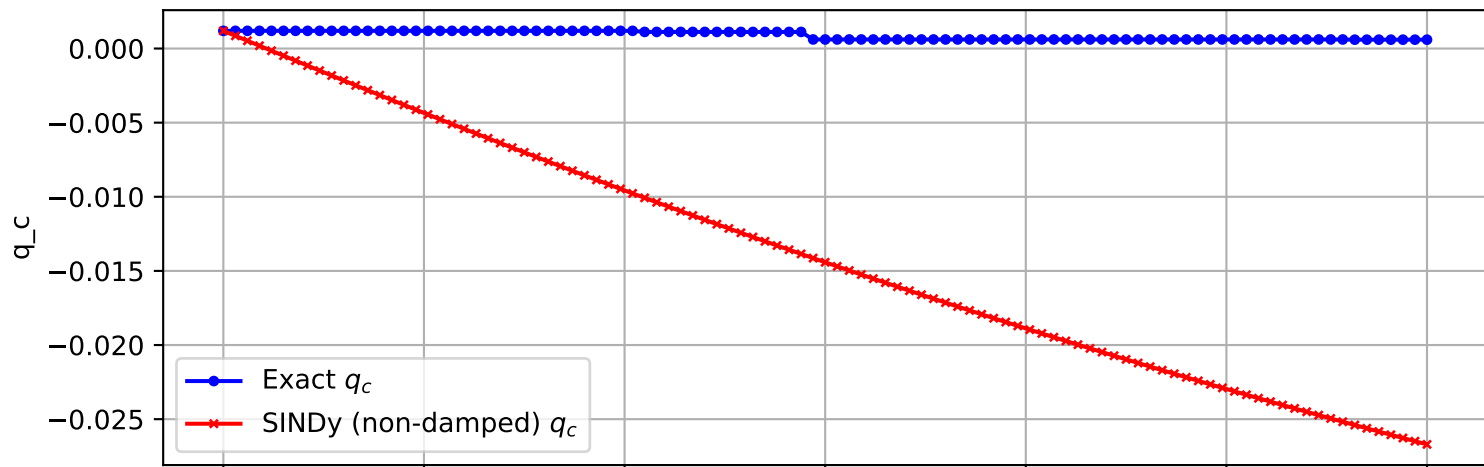
Trajectory 492 (non-damped)
