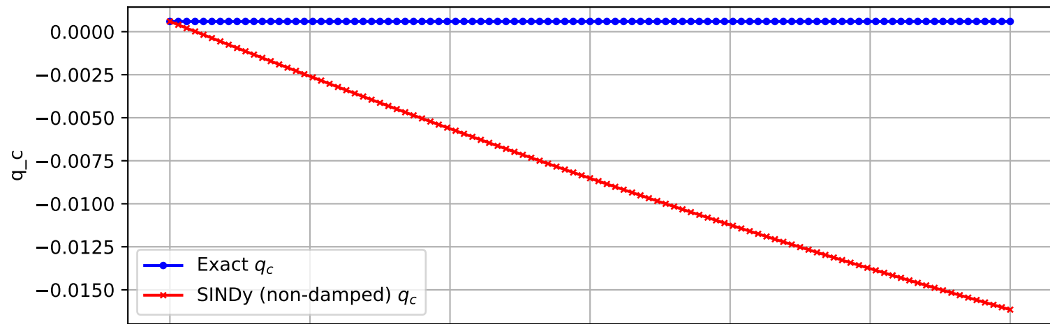
Trajectory 495 (non-damped)
