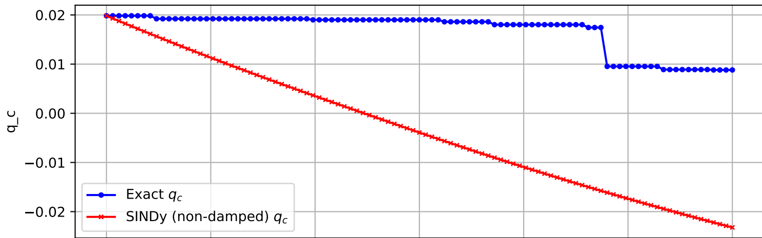
Trajectory 5 (non-damped)
