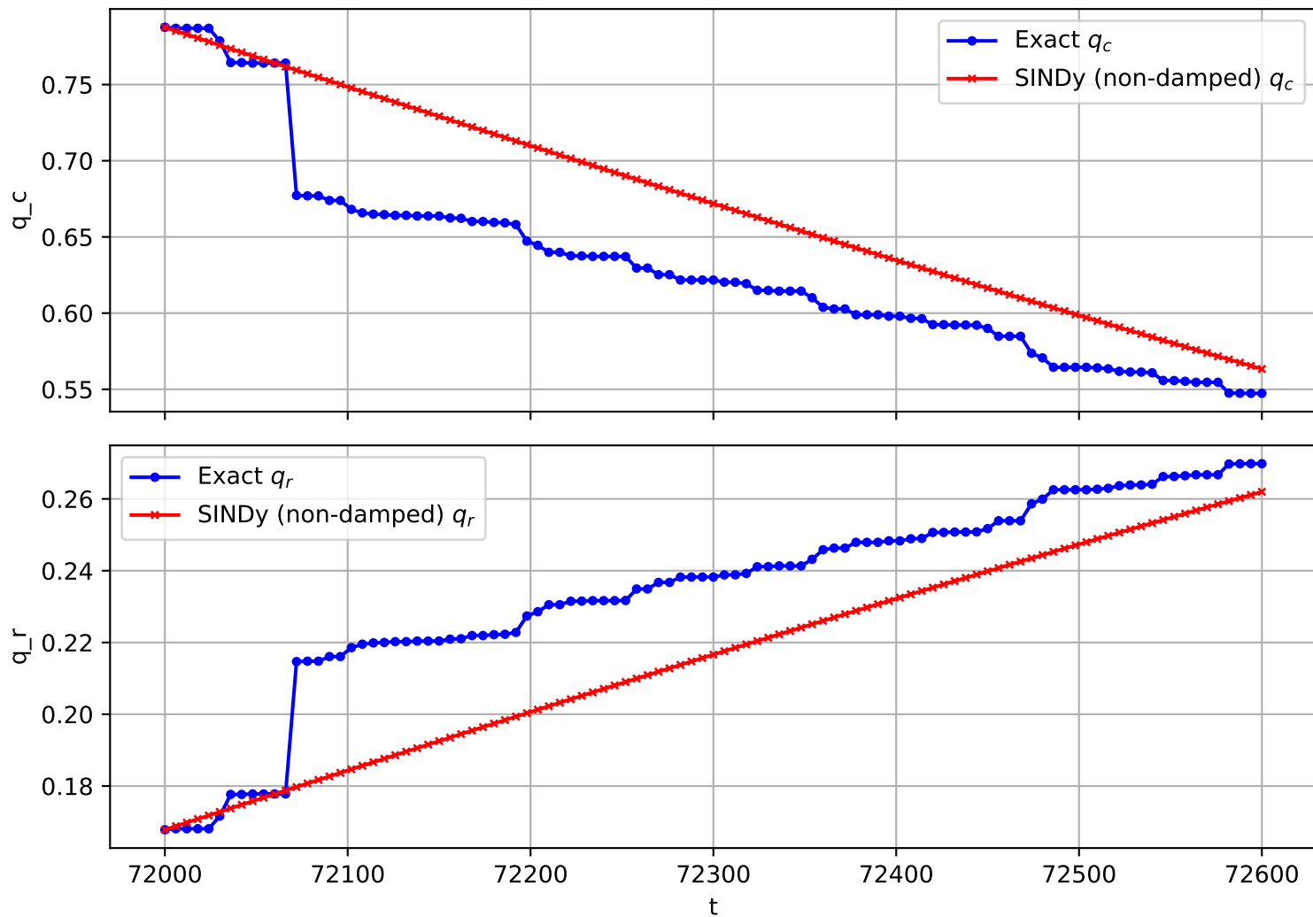
Trajectory 507 (non-damped)
