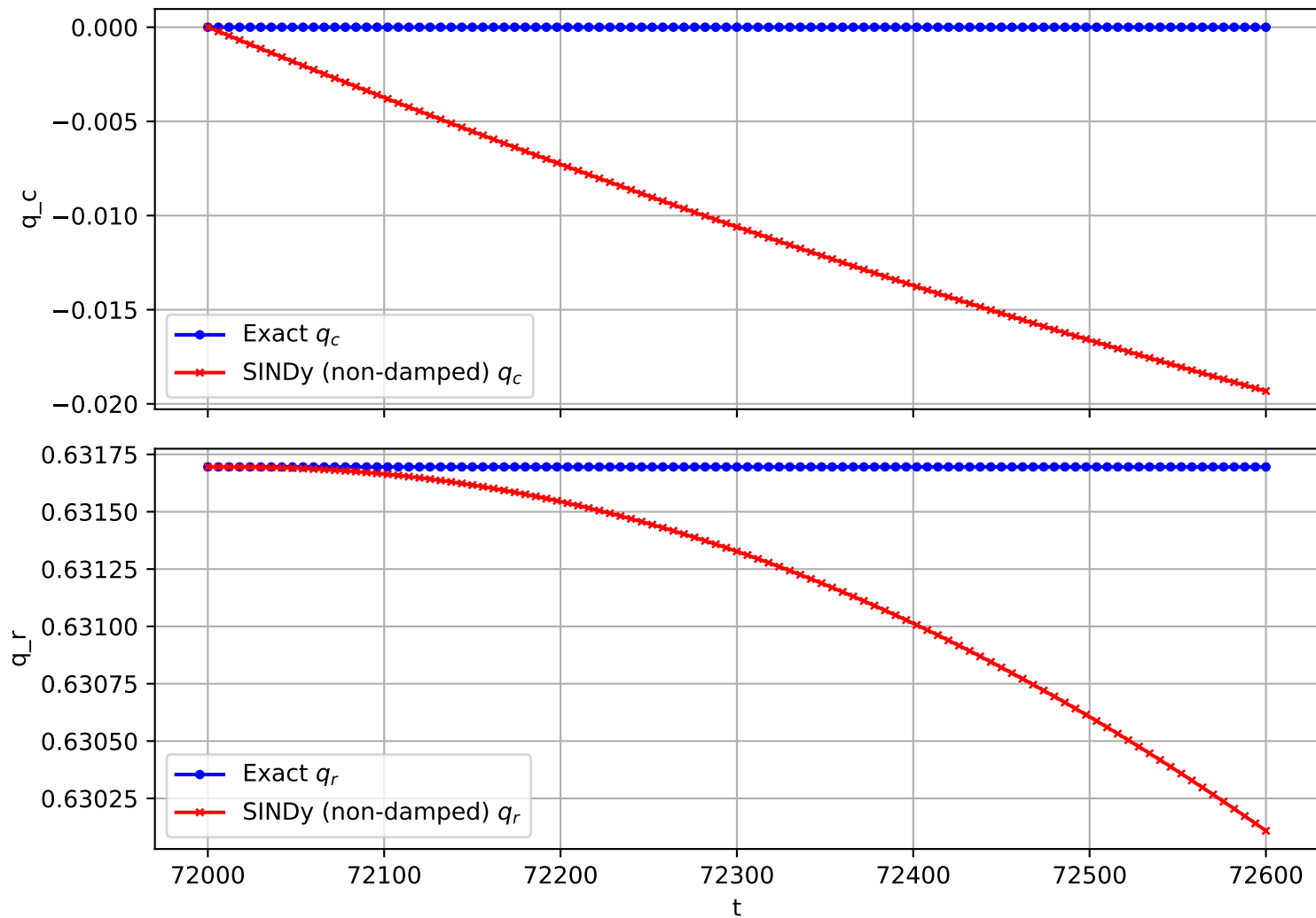
Trajectory 513 (non-damped)
