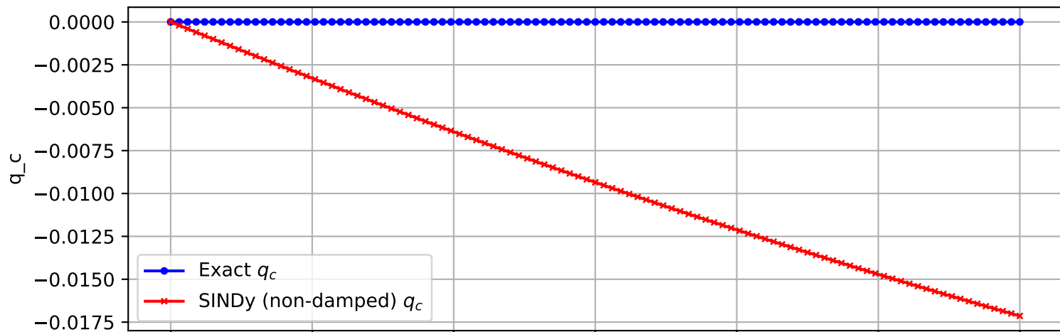
Trajectory 514 (non-damped)
