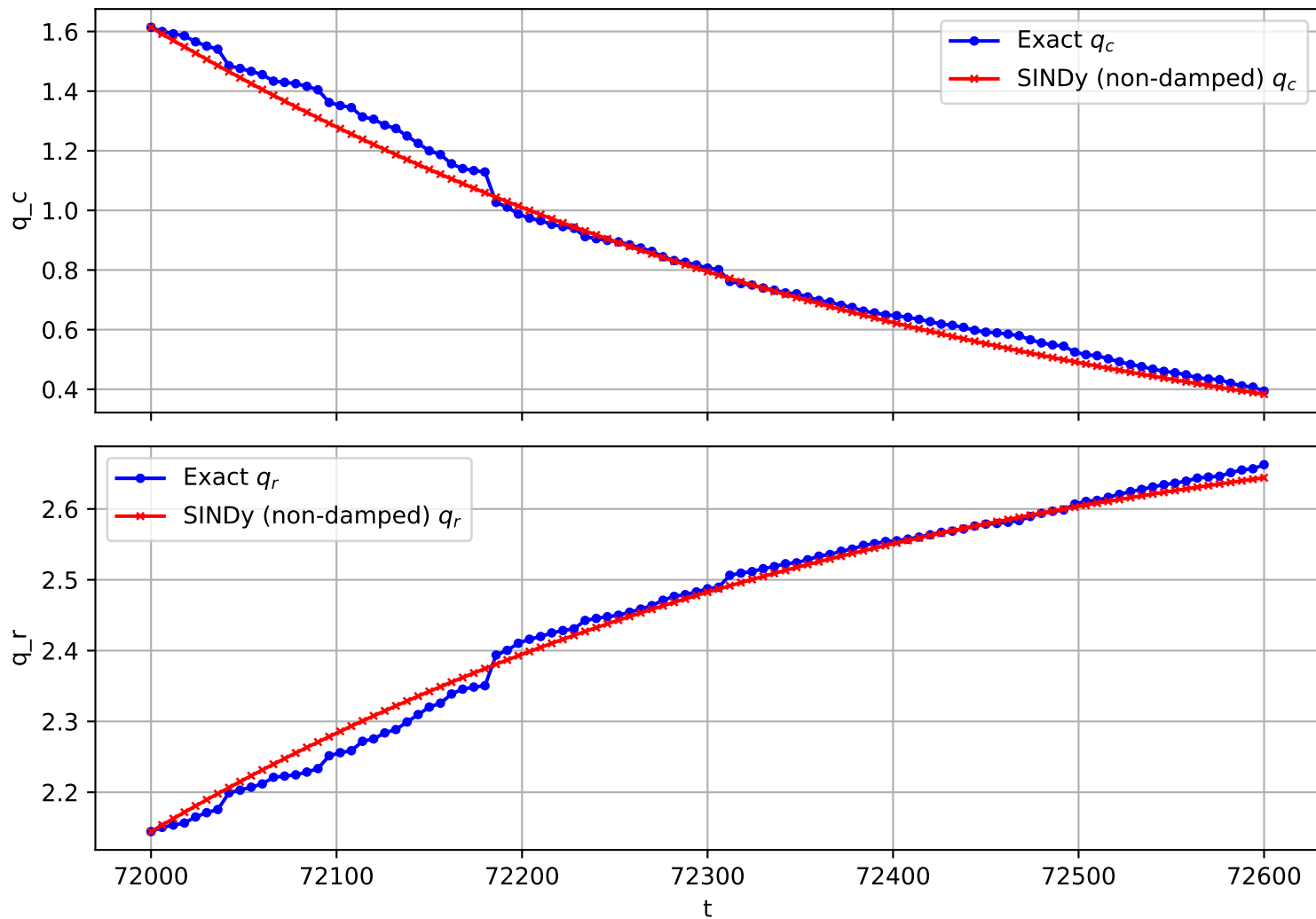
Trajectory 528 (non-damped)
