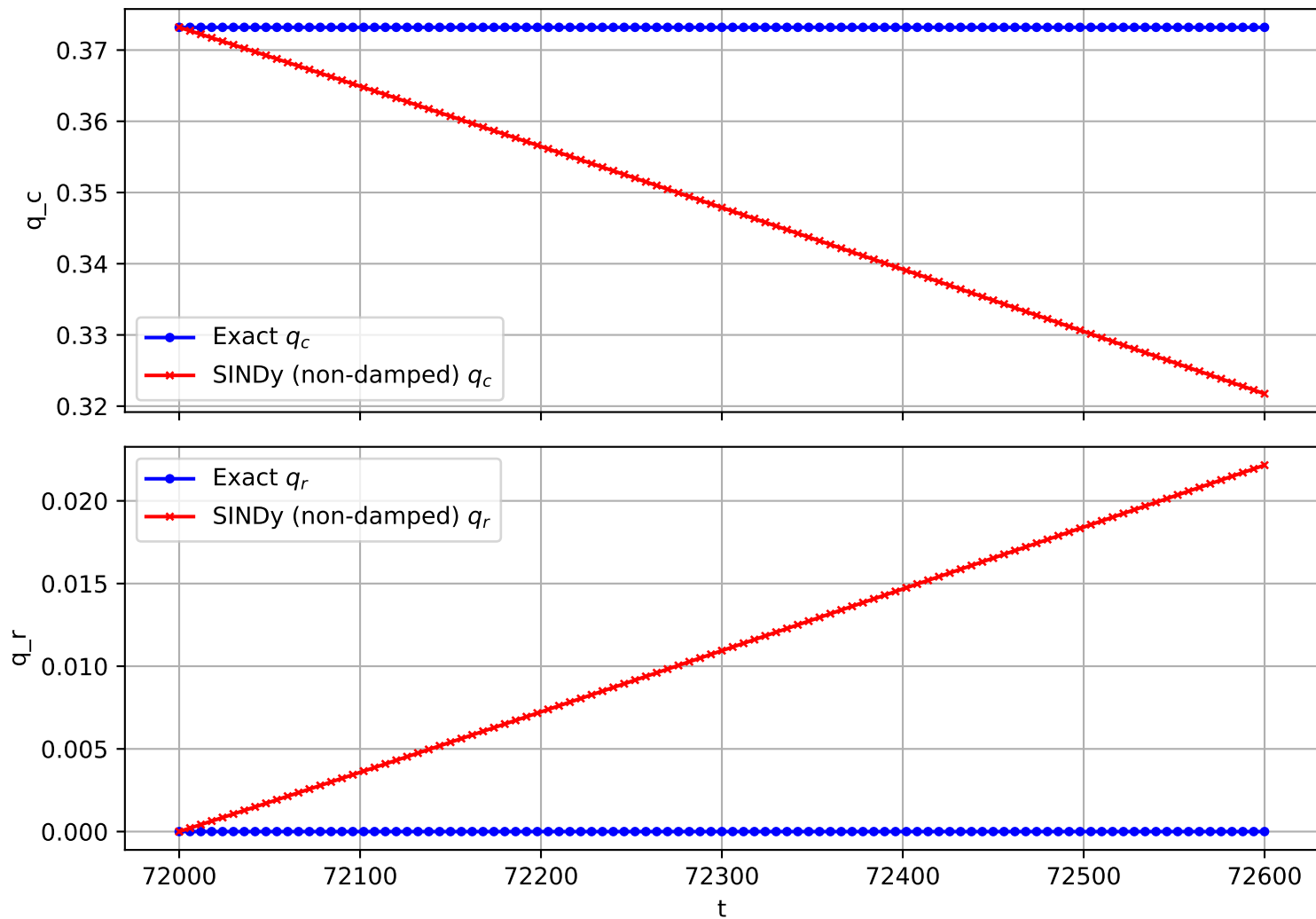
Trajectory 53 (non-damped)
