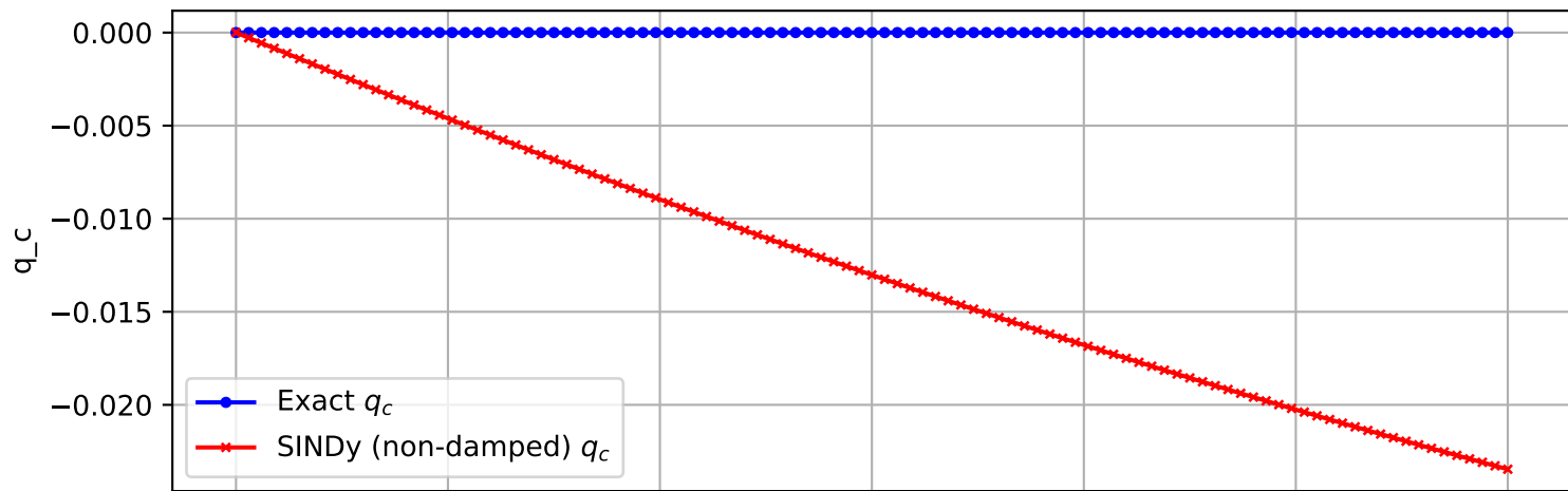
Trajectory 538 (non-damped)
