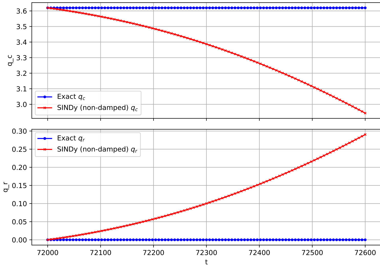
Trajectory 54 (non-damped)
