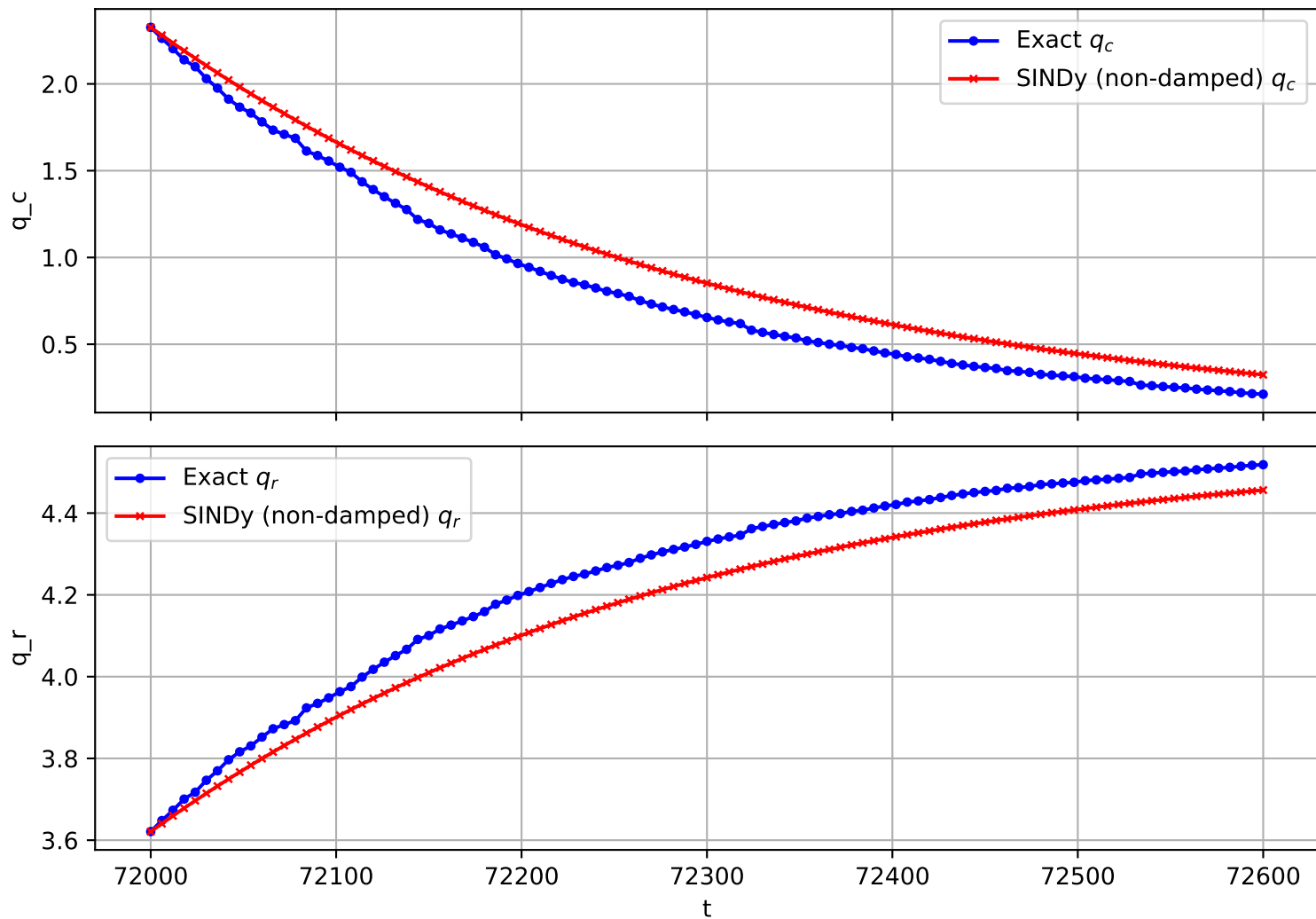
Trajectory 545 (non-damped)
