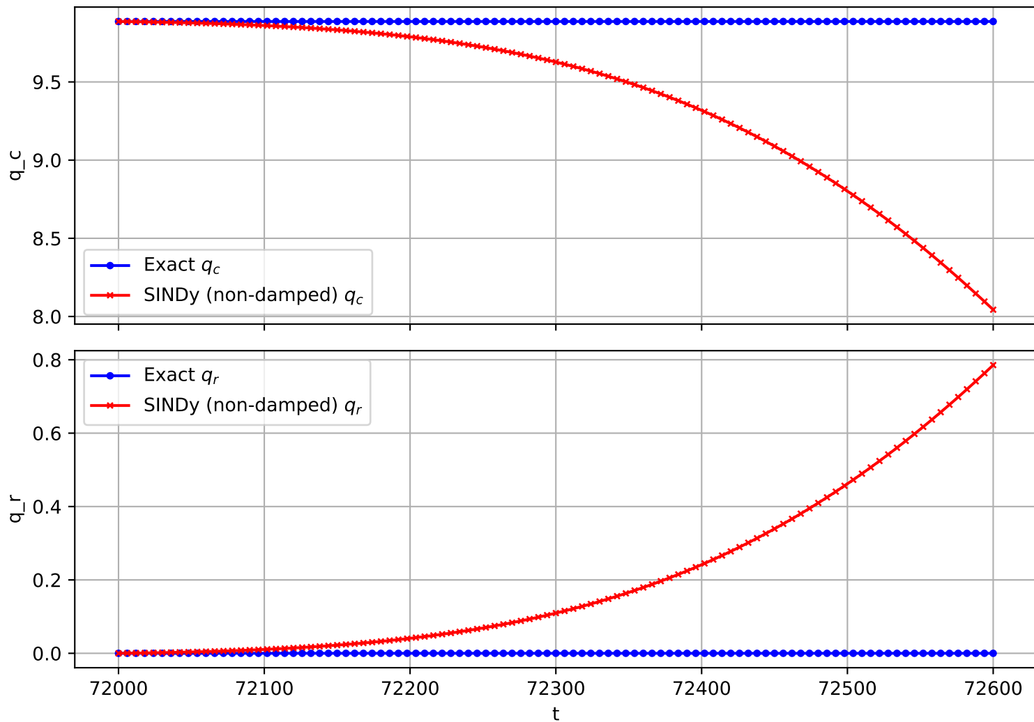
Trajectory 55 (non-damped)
