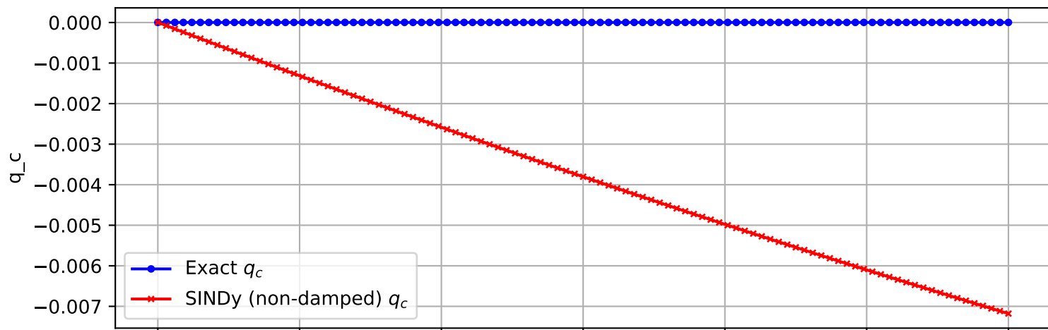
Trajectory 571 (non-damped)
