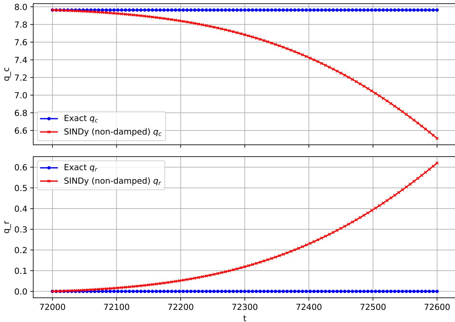
Trajectory 58 (non-damped)
