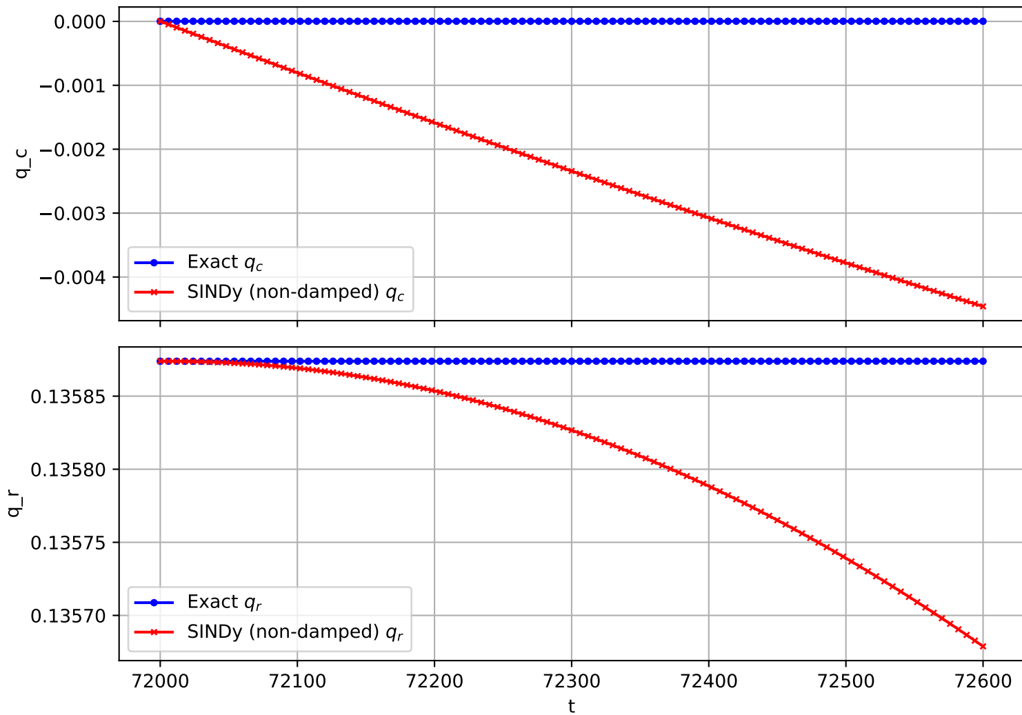
Trajectory 580 (non-damped)
