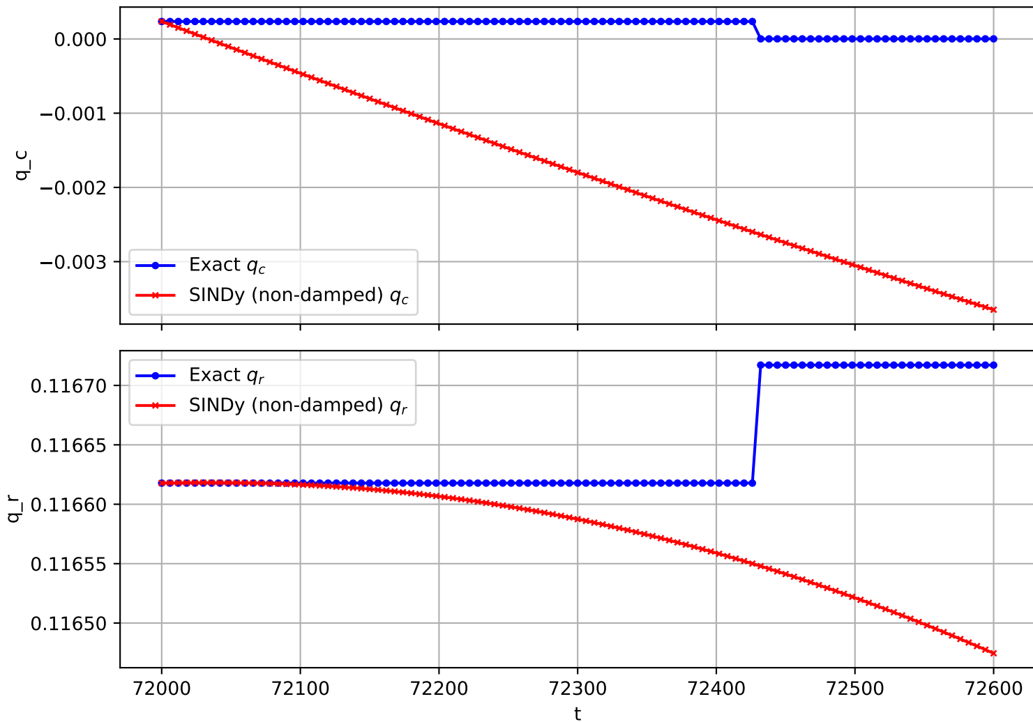
Trajectory 583 (non-damped)
