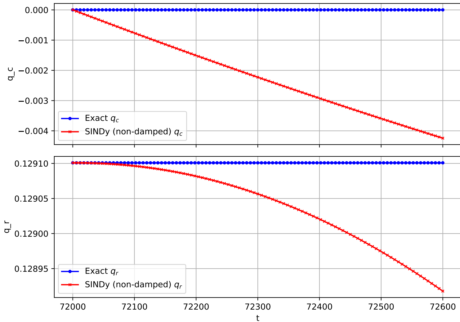
Trajectory 586 (non-damped)
