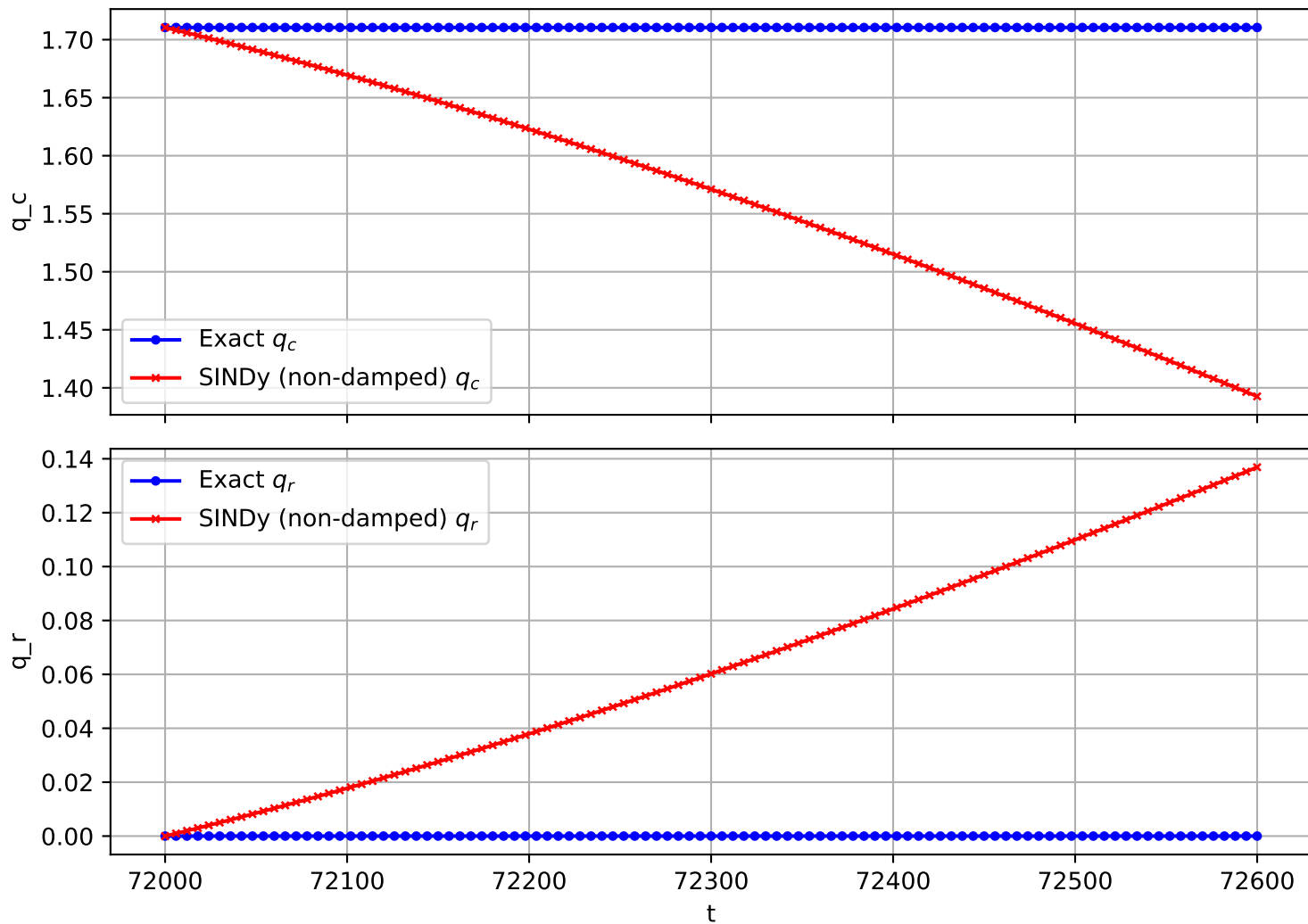
Trajectory 588 (non-damped)
