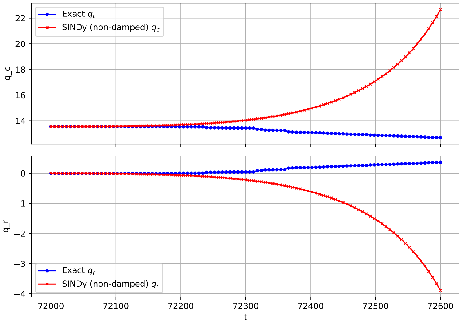
Trajectory 59 (non-damped)
