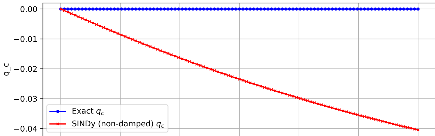
Trajectory 601 (non-damped)
