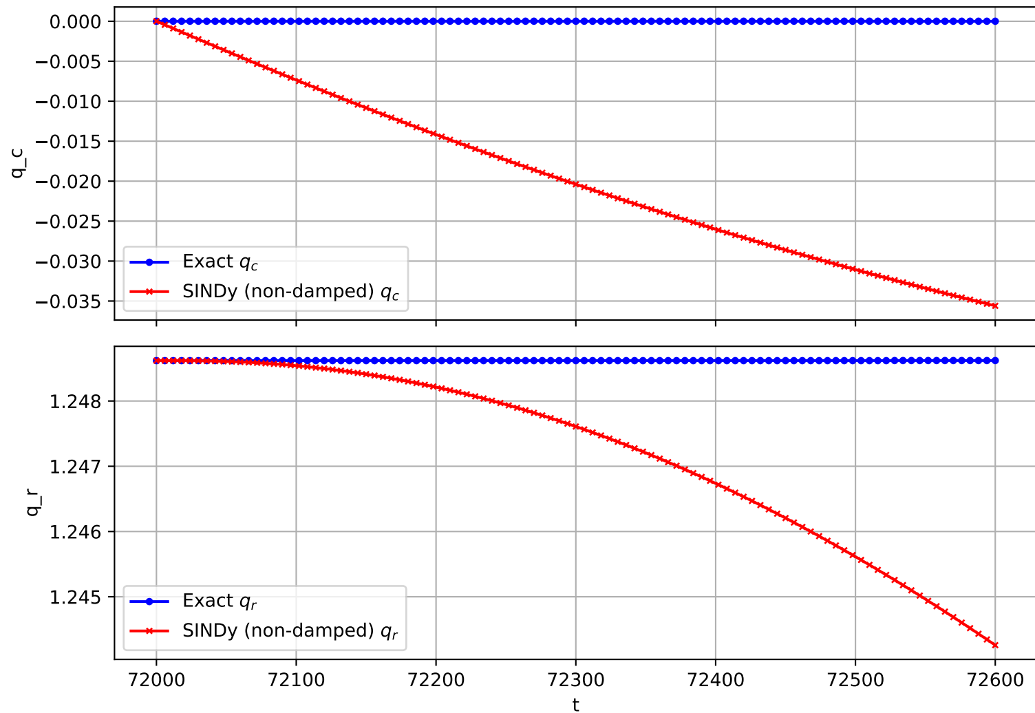
Trajectory 605 (non-damped)
