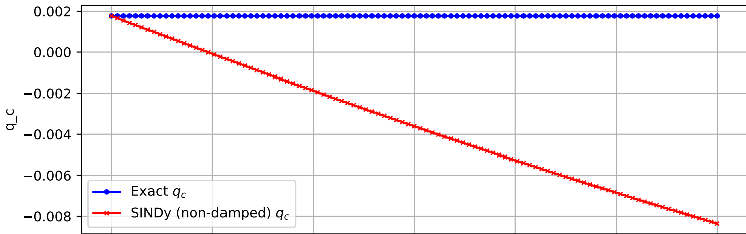
Trajectory 607 (non-damped)
