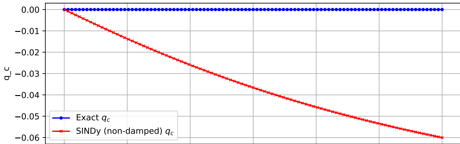
Trajectory 609 (non-damped)
